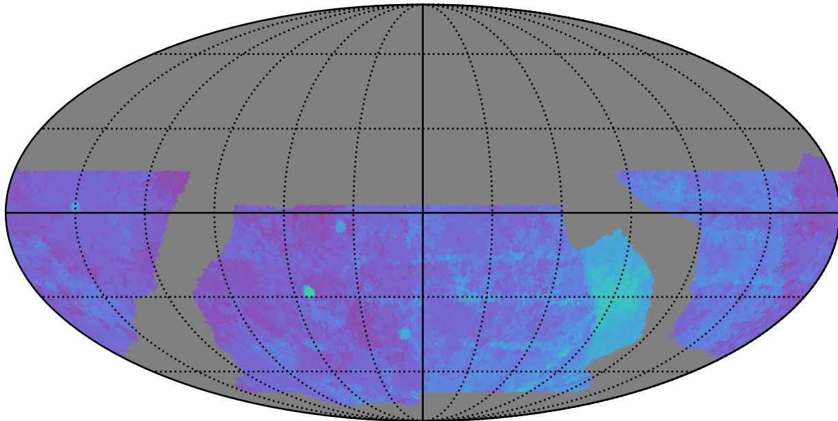
baseline_v2.1_10yrs WFD g band: 80thPercentile Season Length
