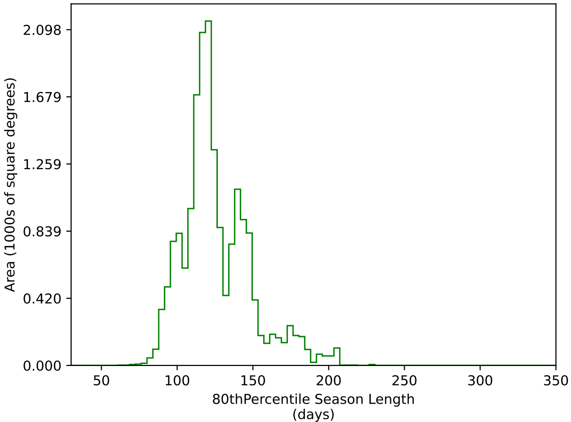
baseline_v2.1_10yrs WFD g band: 80thPercentile Season Length
