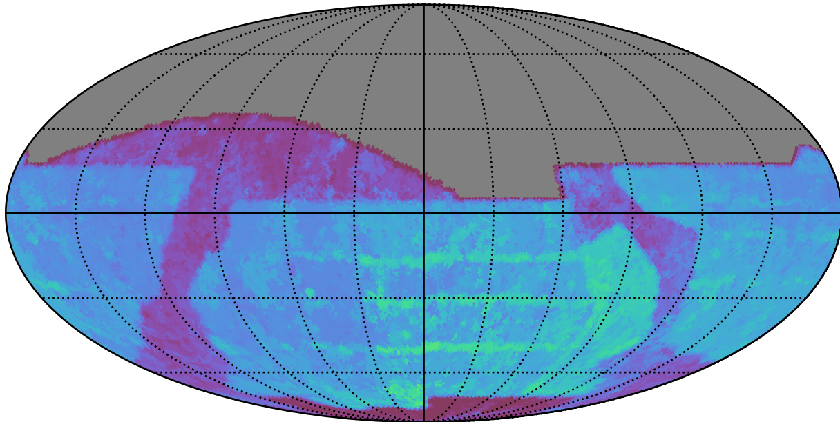
baseline_v2.1_10yrs All sky z band: 80thPercentile Season Length
