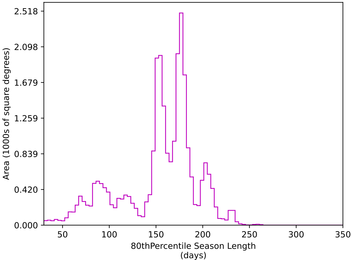
baseline_v2.1_10yrs All sky z band: 80thPercentile Season Length
