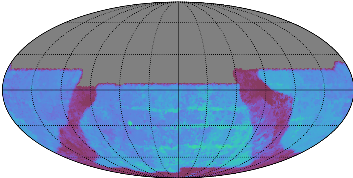
baseline_v2.1_10yrs All sky y band: 80thPercentile Season Length
