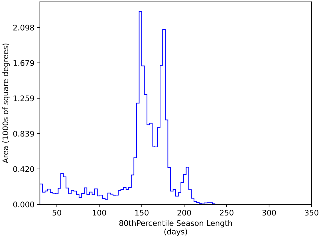
baseline_v2.1_10yrs All sky y band: 80thPercentile Season Length
