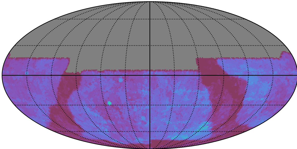
baseline_v2.1_10yrs All sky u band: 80thPercentile Season Length
