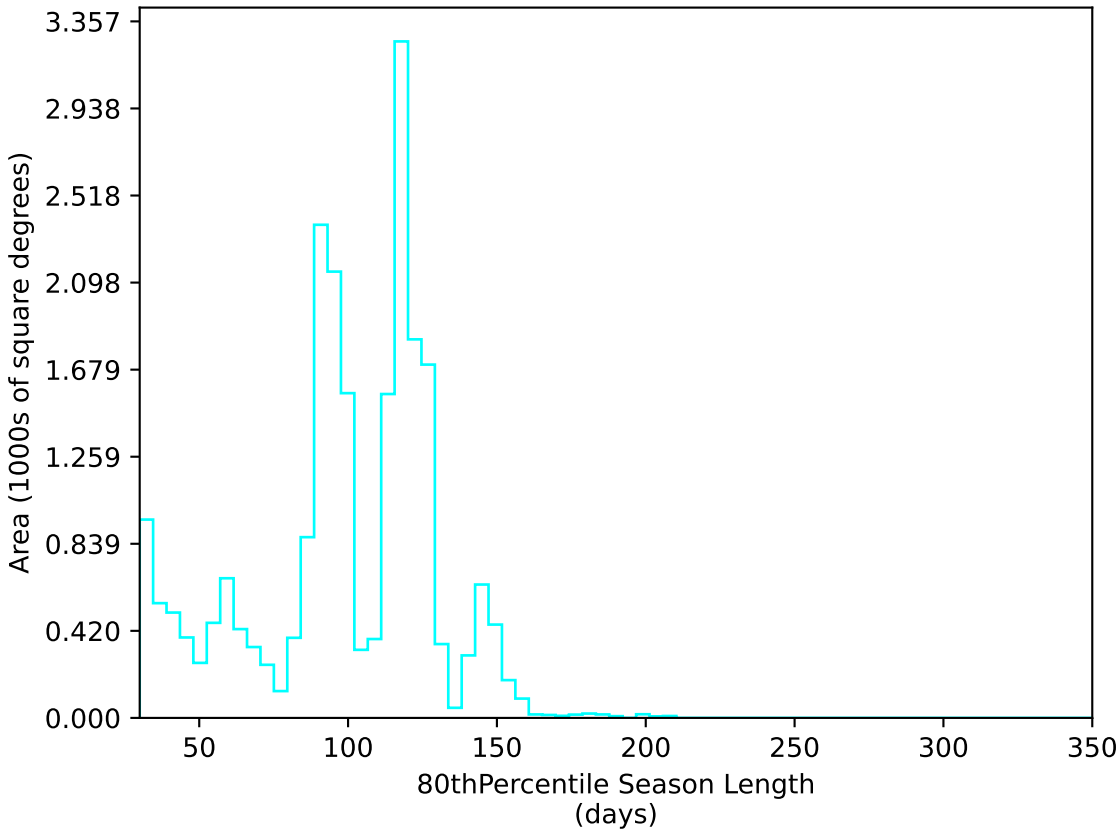
baseline_v2.1_10yrs All sky u band: 80thPercentile Season Length
