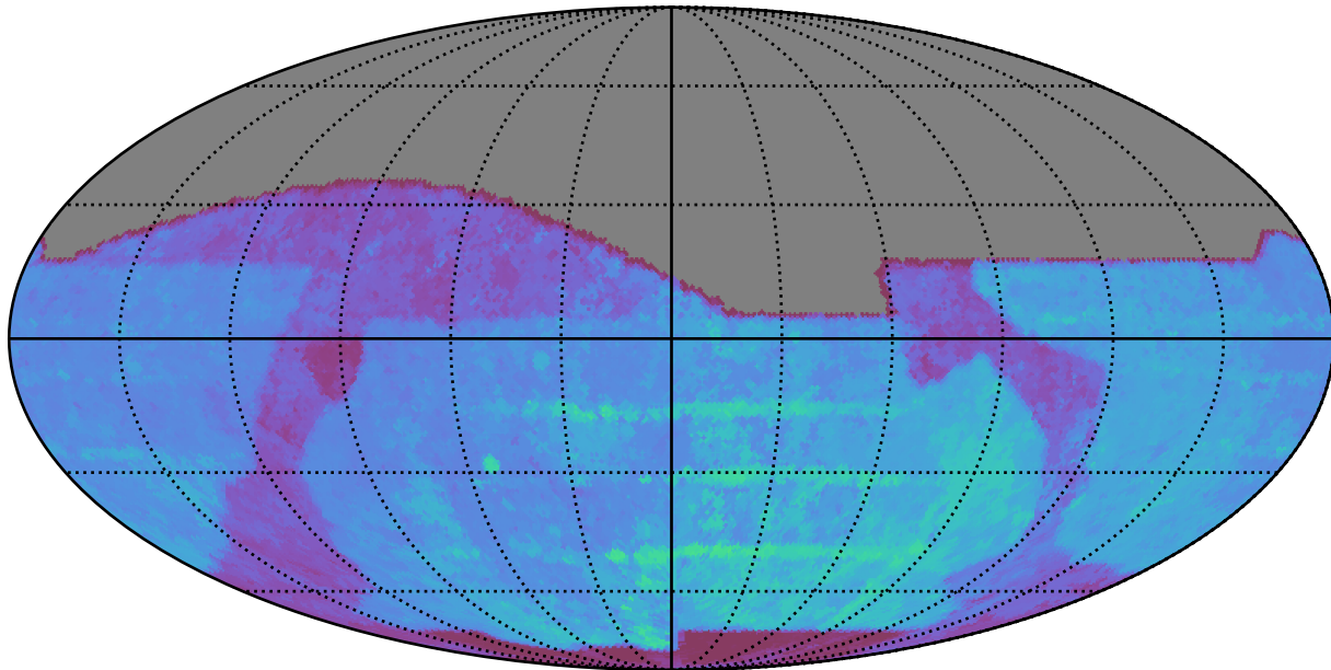
baseline_v2.1_10yrs All sky r band: 80thPercentile Season Length
