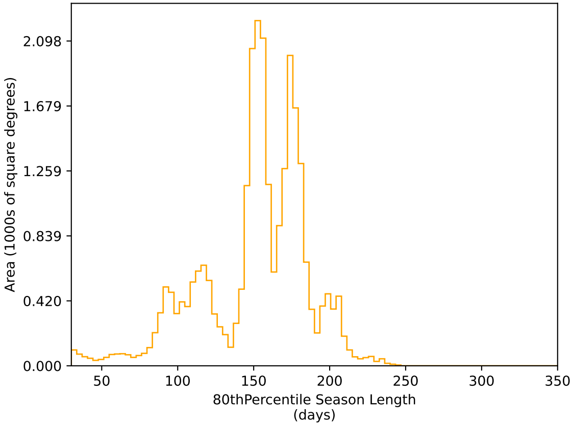
baseline_v2.1_10yrs All sky r band: 80thPercentile Season Length
