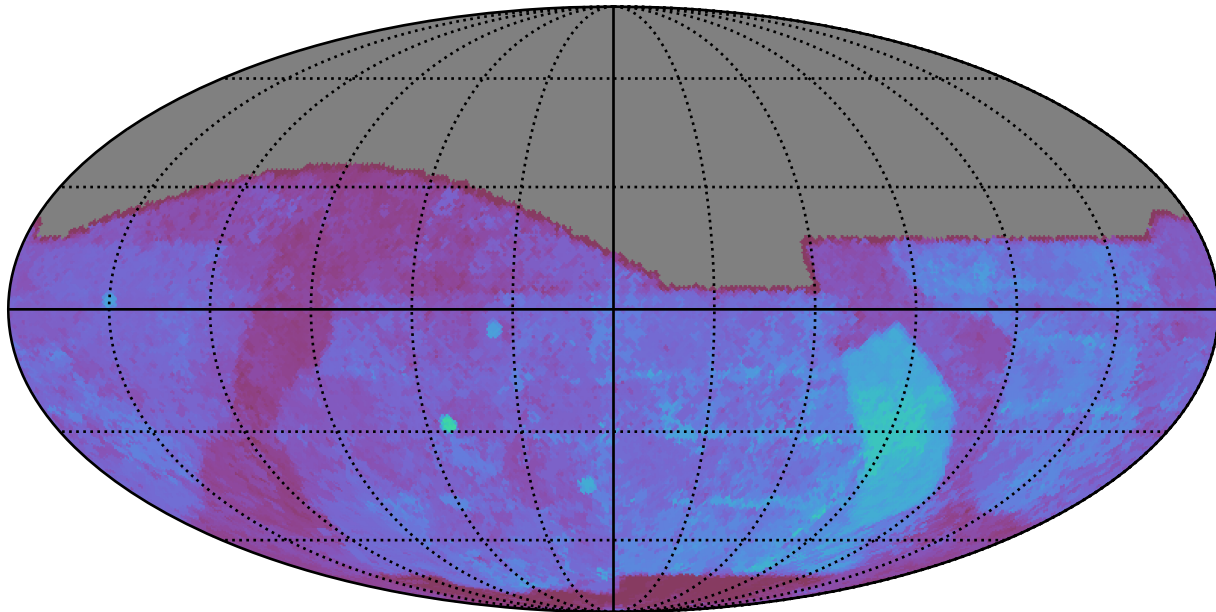
baseline_v2.1_10yrs All sky g band: 80thPercentile Season Length
