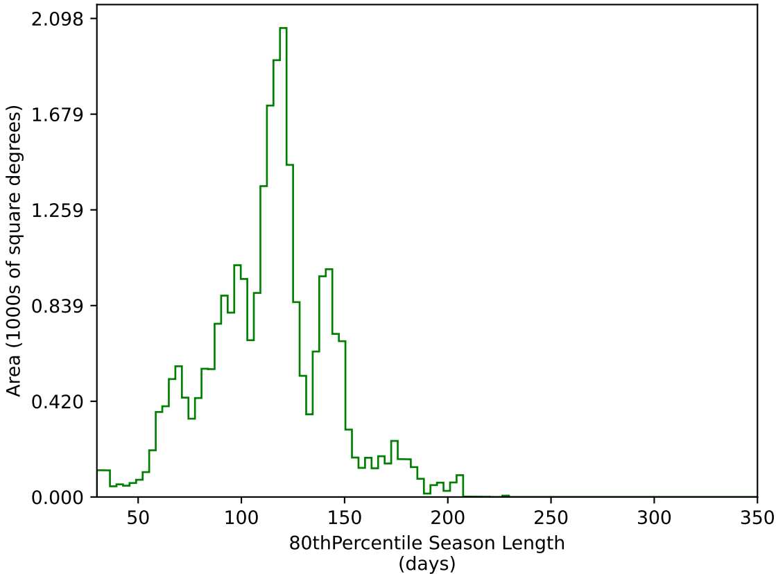
baseline_v2.1_10yrs All sky g band: 80thPercentile Season Length
