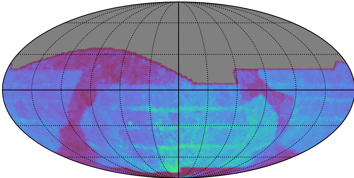
baseline_v2.1_10yrs All sky all bands: 80thPercentile Season Length
