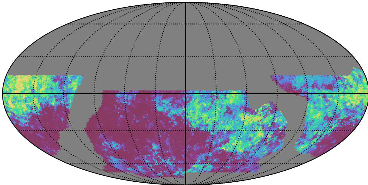
baseline_v2.1_10yrs WFD zy bands: 75th Percentile Intranight Timespan
