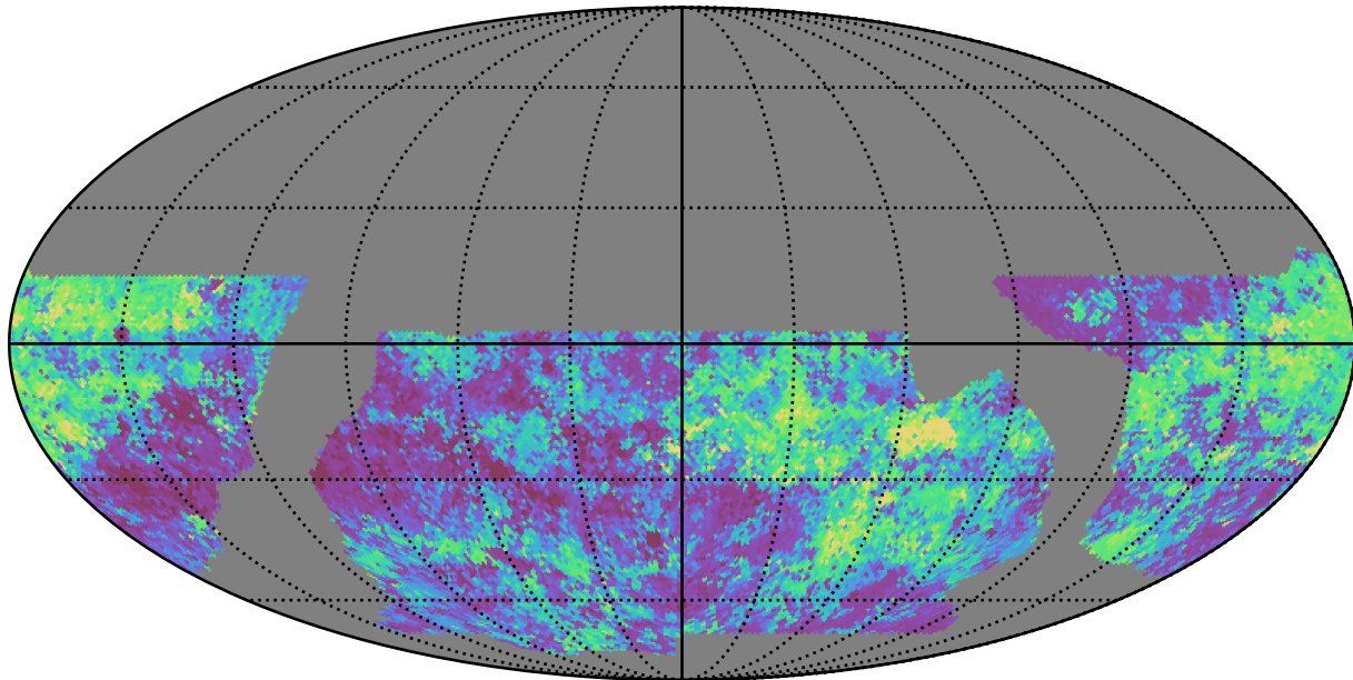
baseline_v2.1_10yrs WFD z band: 75th Percentile Intranight Timespan
