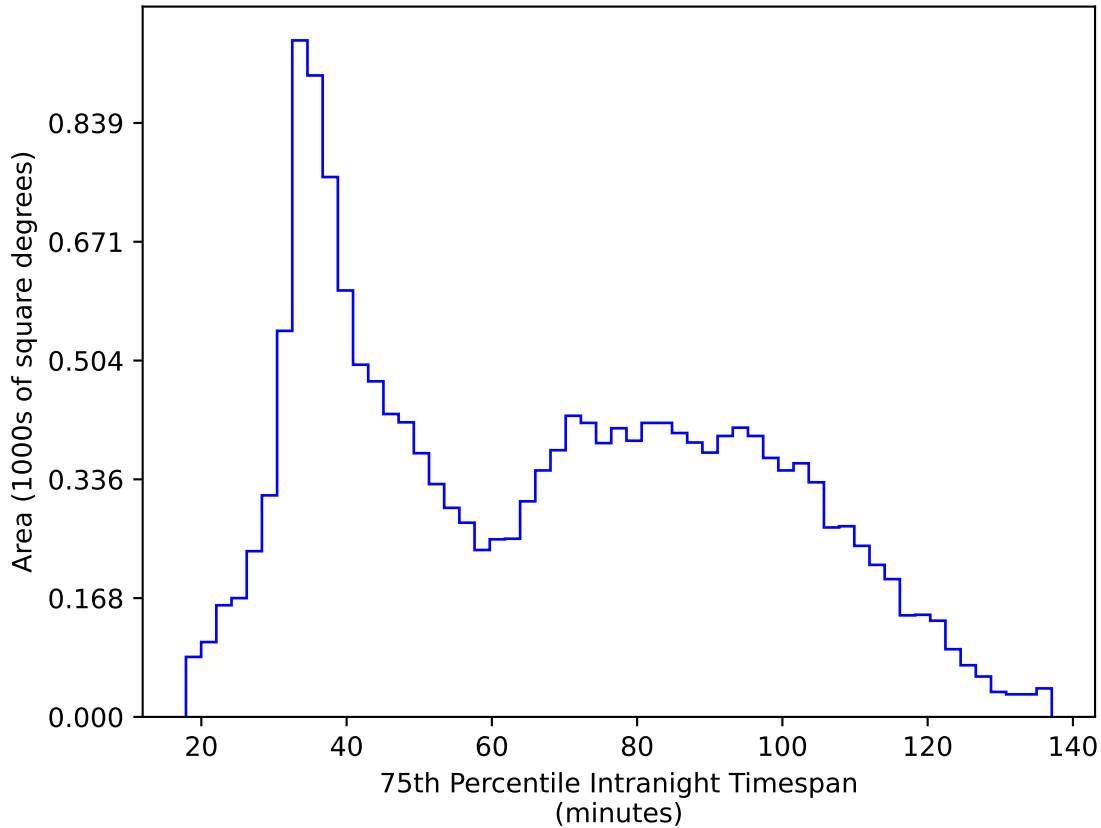
baseline_v2.1_10yrs WFD z band: 75th Percentile Intranight Timespan
