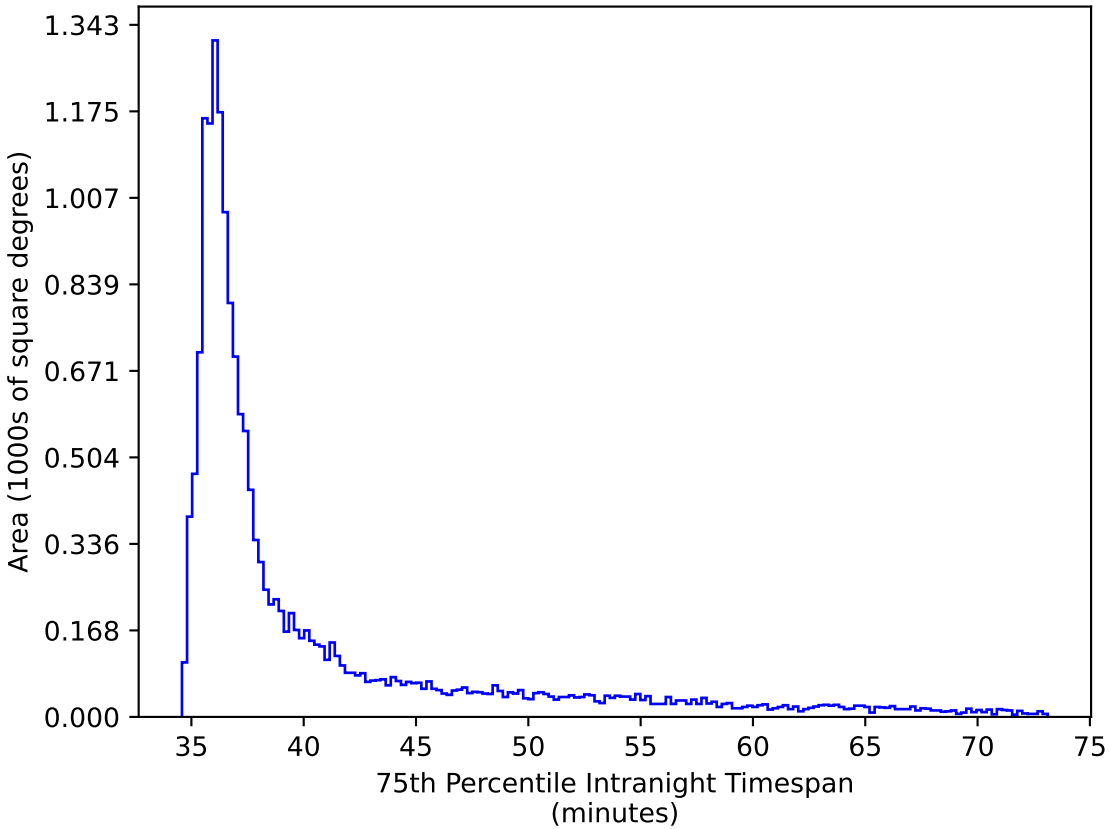
baseline_v2.1_10yrs WFD ri bands: 75th Percentile Intranight Timespan
