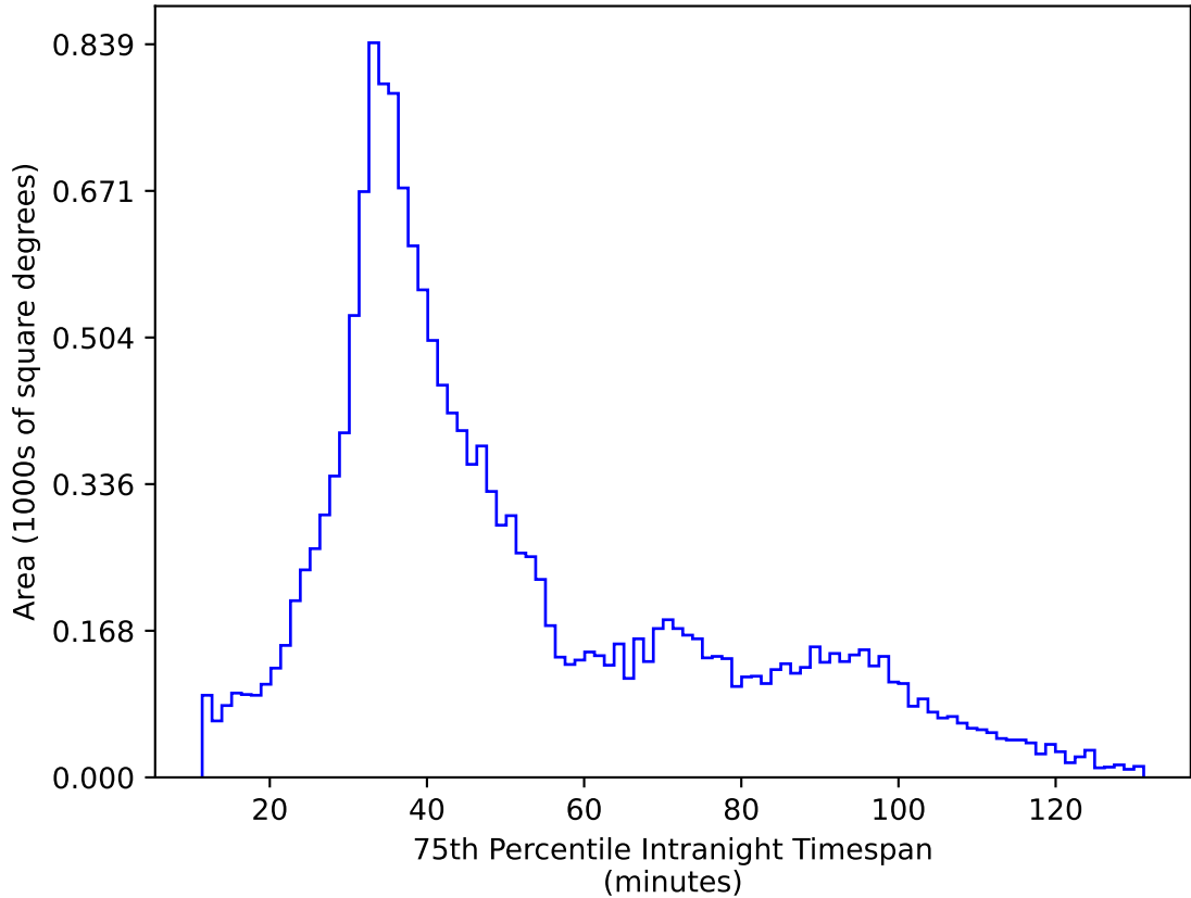
baseline_v2.1_10yrs WFD r band: 75th Percentile Intranight Timespan
