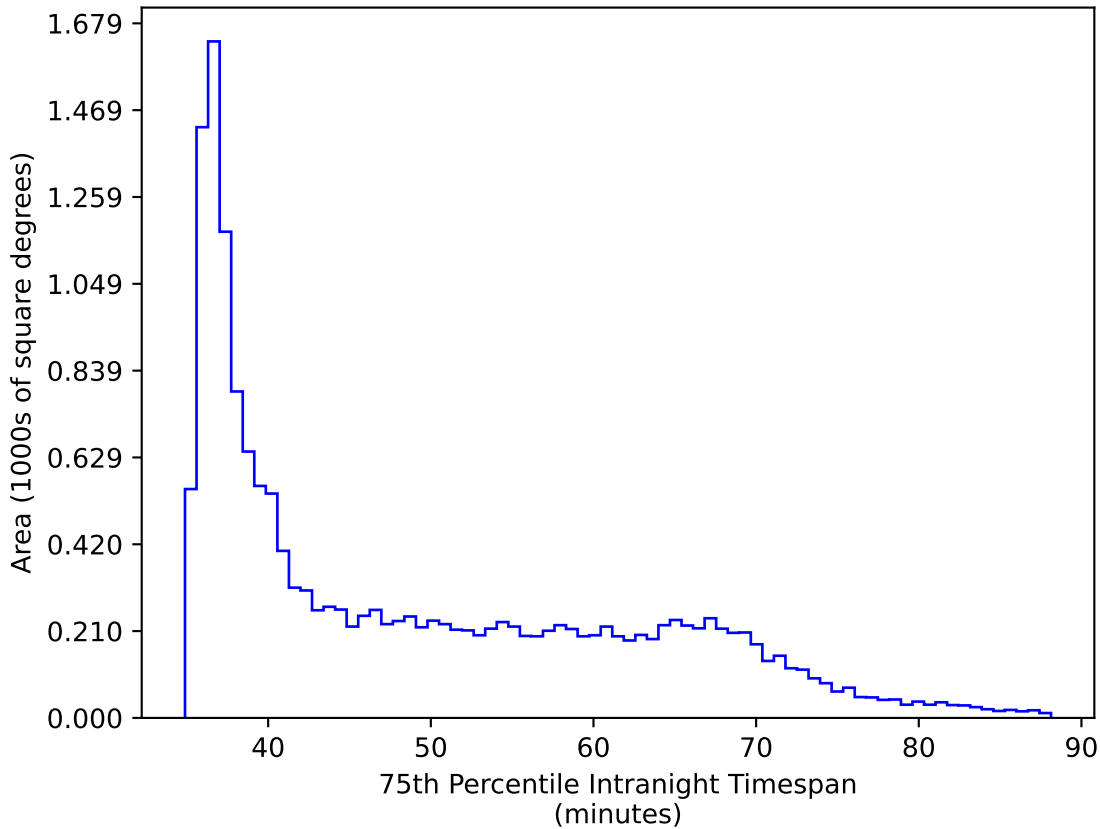
baseline_v2.1_10yrs WFD gr bands: 75th Percentile Intranight Timespan
