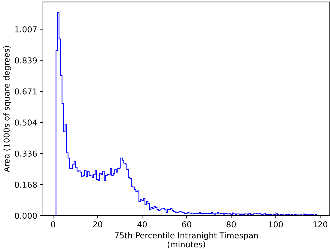
baseline_v2.1_10yrs WFD g band: 75th Percentile Intranight Timespan
