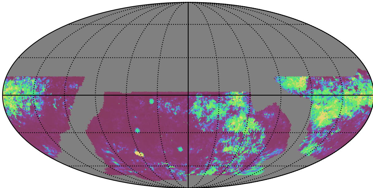
baseline_v2.1_10yrs WFD all bands: 75th Percentile Intranight Timespan
