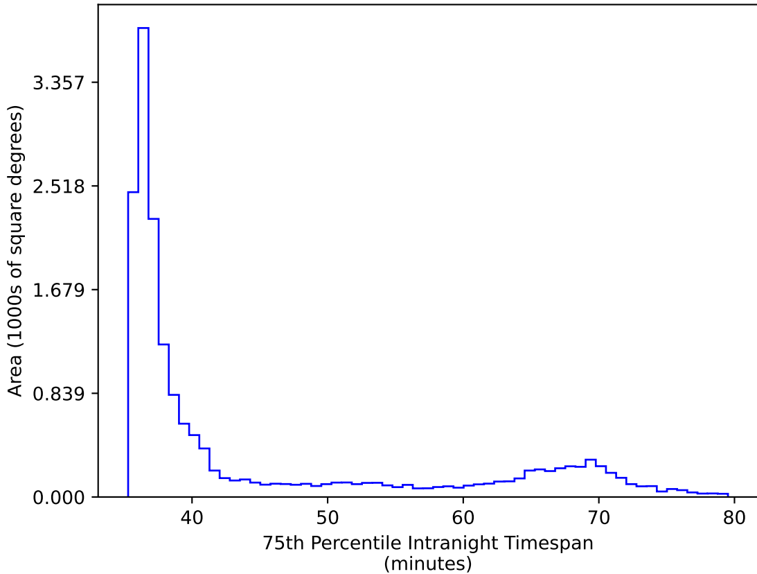
baseline_v2.1_10yrs WFD all bands: 75th Percentile Intranight Timespan
