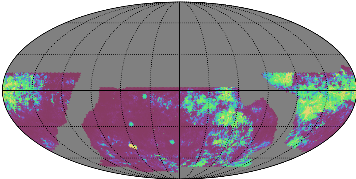
baseline_v2.1_10yrs WFD: 75th Percentile Intranight Timespan
