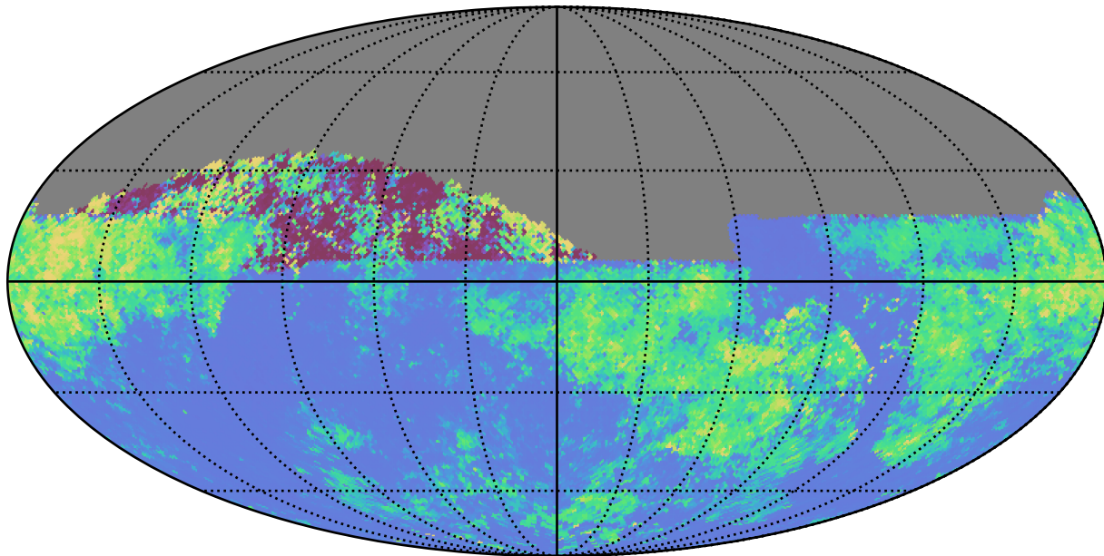
baseline_v2.1_10yrs All sky zy bands: 75th Percentile Intranight Timespan
