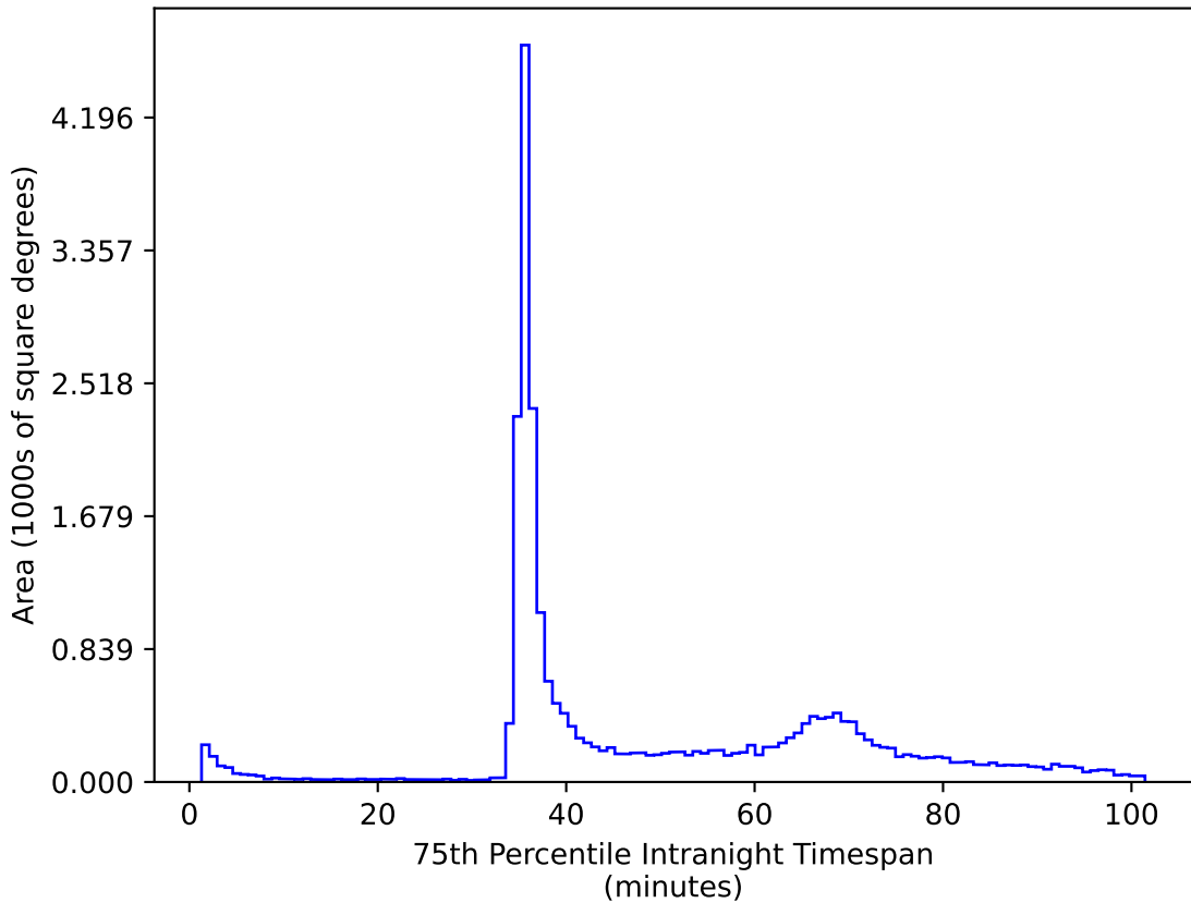
baseline_v2.1_10yrs All sky zy bands: 75th Percentile Intranight Timespan
