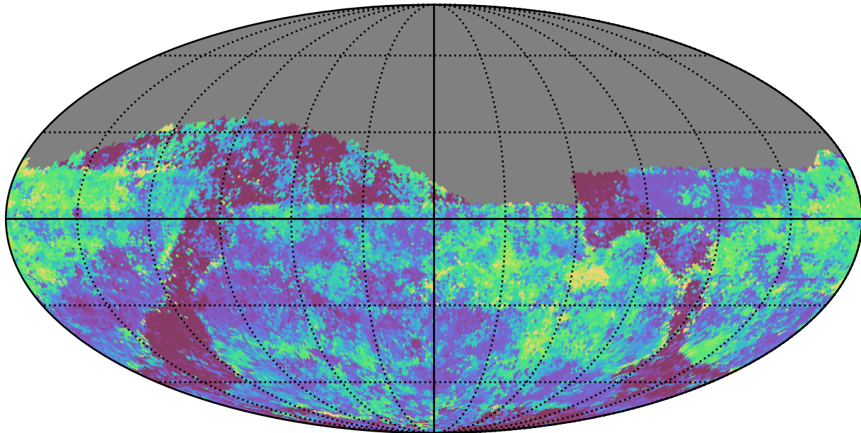
baseline_v2.1_10yrs All sky z band: 75th Percentile Intranight Timespan
