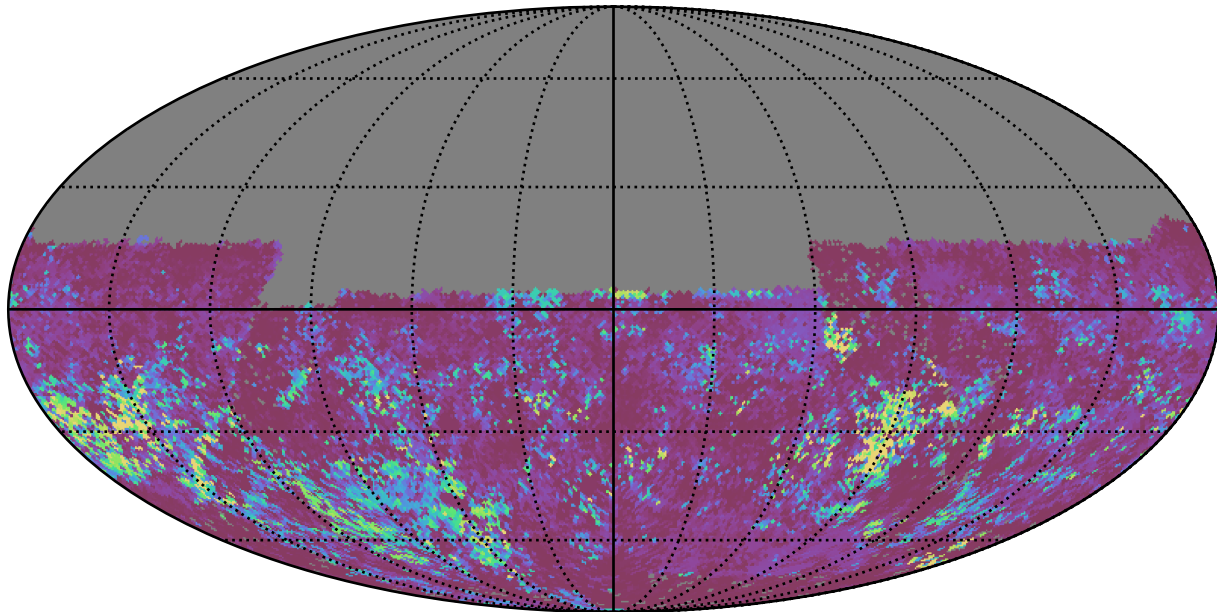
baseline_v2.1_10yrs All sky u band: 75th Percentile Intranight Timespan
