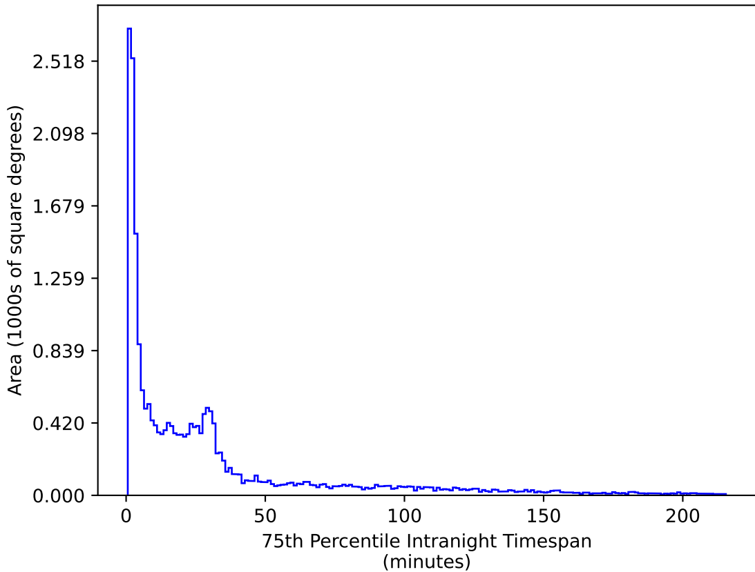
baseline_v2.1_10yrs All sky u band: 75th Percentile Intranight Timespan
