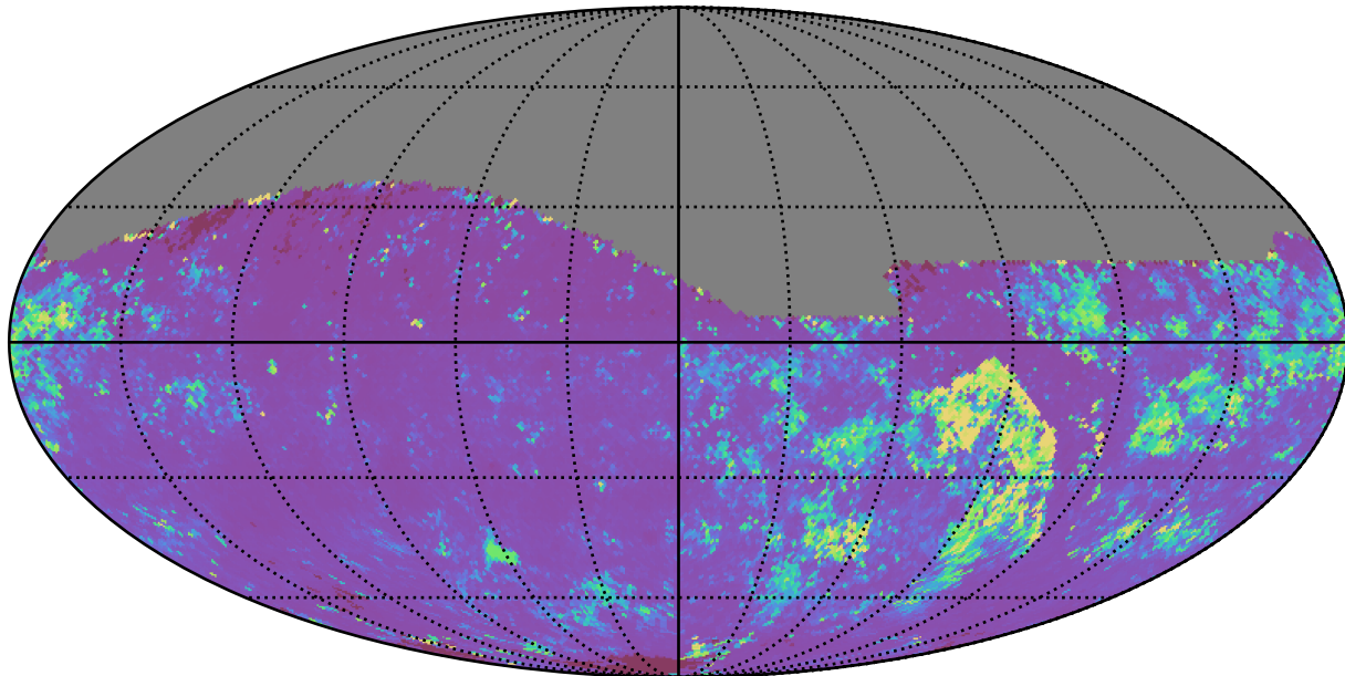
baseline_v2.1_10yrs All sky ri bands: 75th Percentile Intranight Timespan
