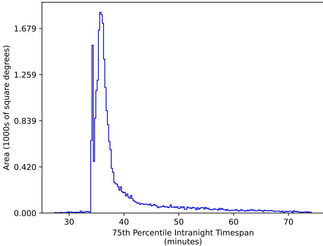
baseline_v2.1_10yrs All sky ri bands: 75th Percentile Intranight Timespan
