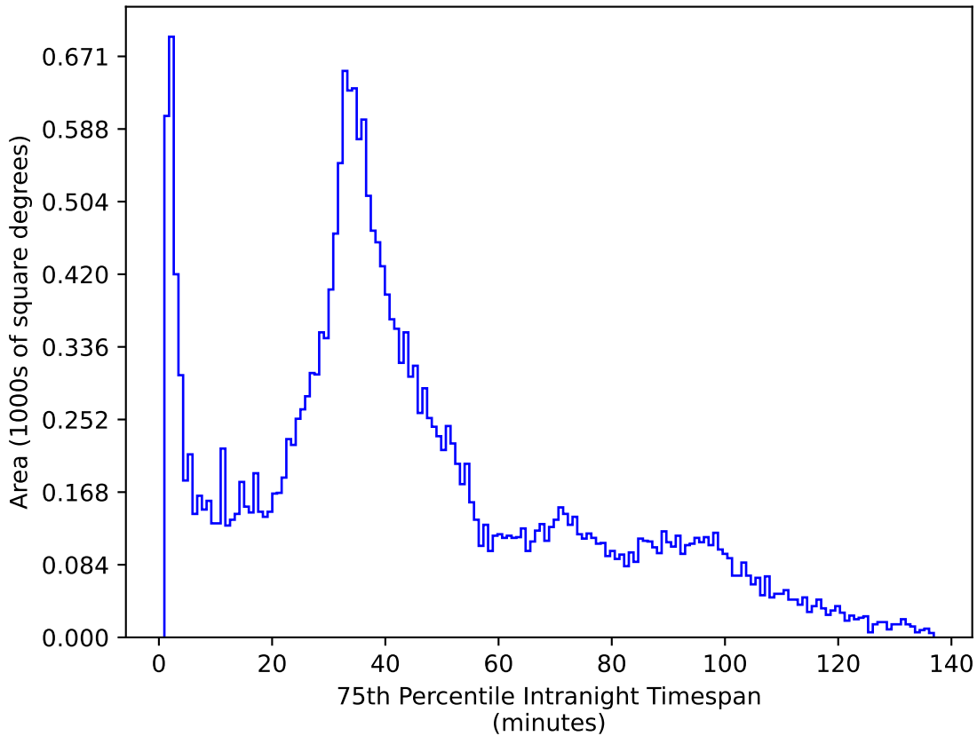
baseline_v2.1_10yrs All sky r band: 75th Percentile Intranight Timespan
