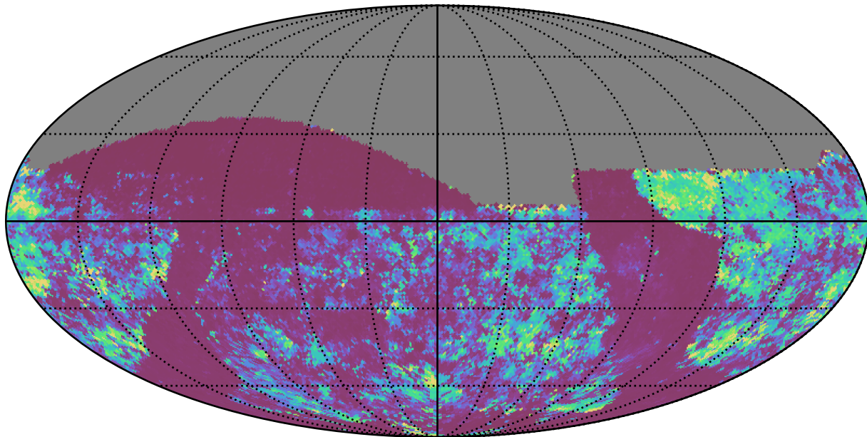
baseline_v2.1_10yrs All sky gr bands: 75th Percentile Intranight Timespan
