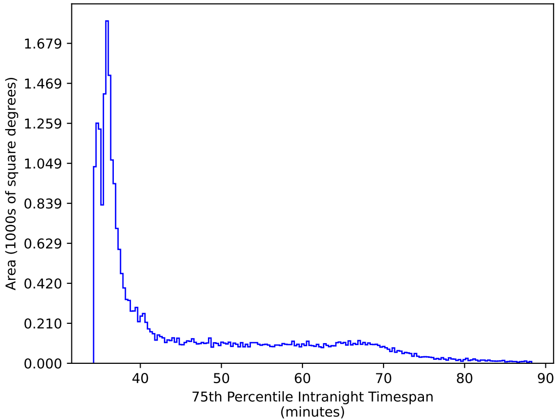
baseline_v2.1_10yrs All sky gr bands: 75th Percentile Intranight Timespan
