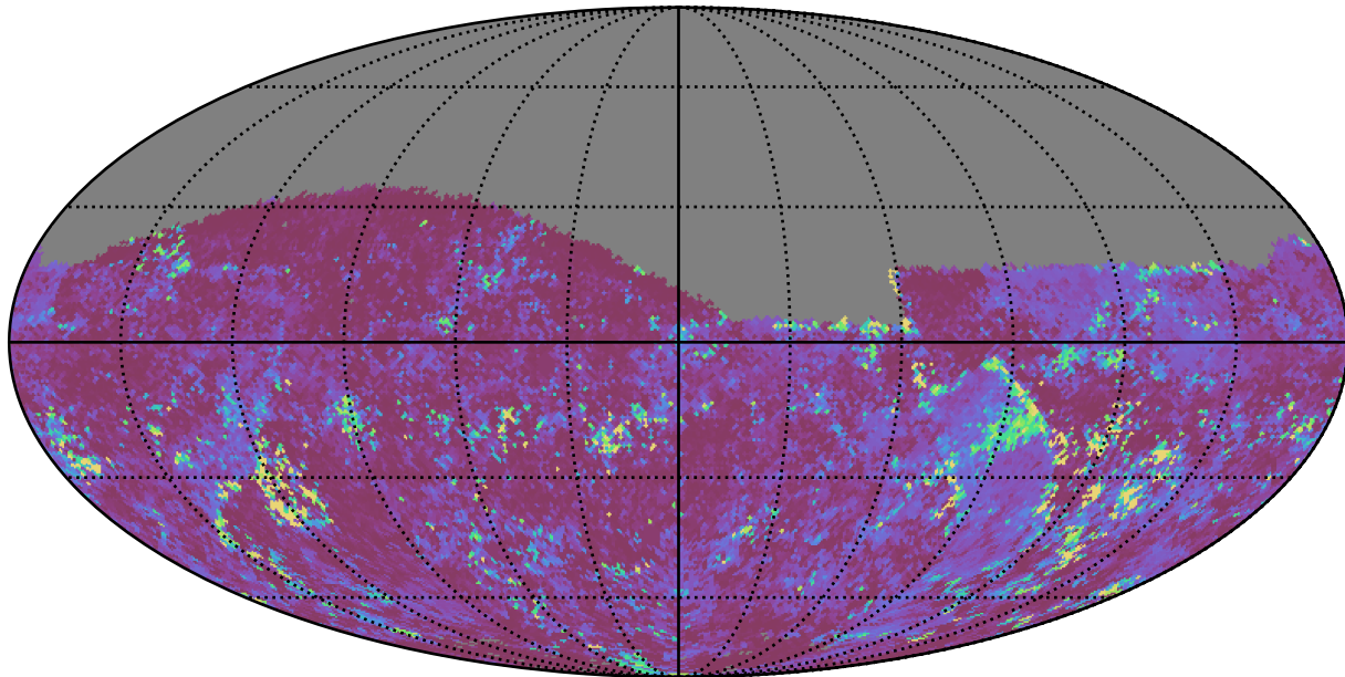
baseline_v2.1_10yrs All sky g band: 75th Percentile Intranight Timespan
