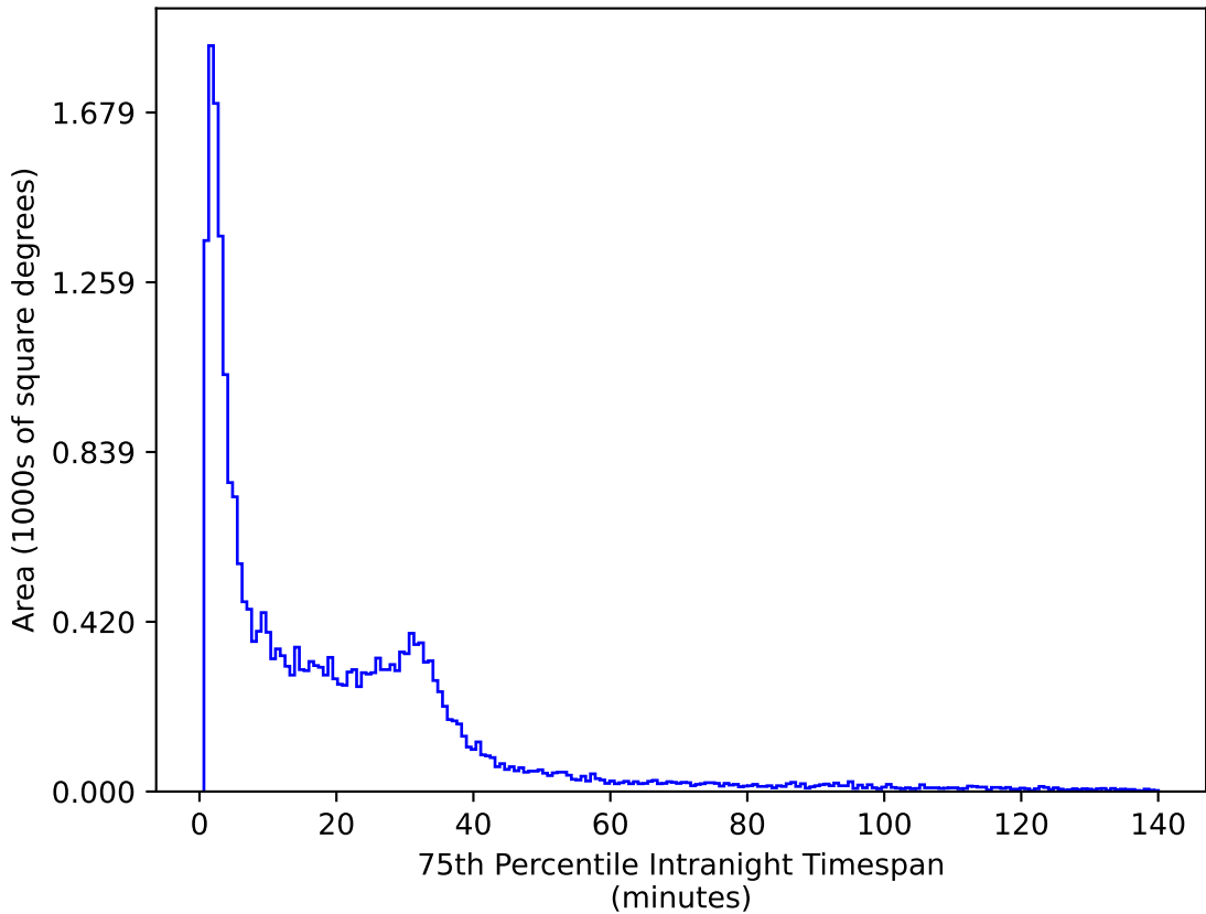
baseline_v2.1_10yrs All sky g band: 75th Percentile Intranight Timespan
