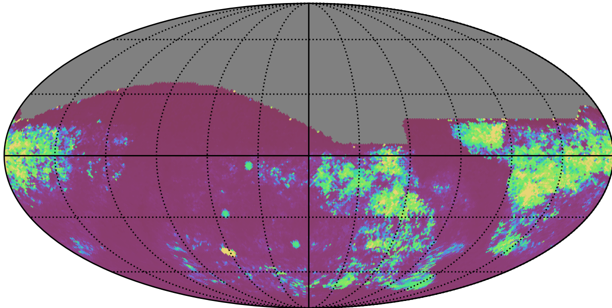
baseline_v2.1_10yrs All sky: 75th Percentile Intranight Timespan
