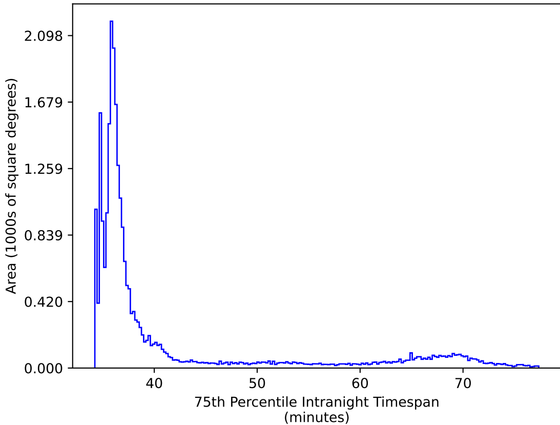
baseline_v2.1_10yrs All sky: 75th Percentile Intranight Timespan
