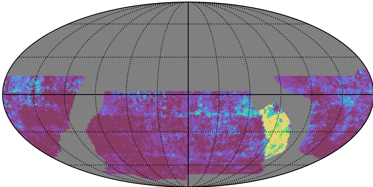
baseline_v2.1_10yrs WFD y band: 20thPercentile Inter-Night Gap
