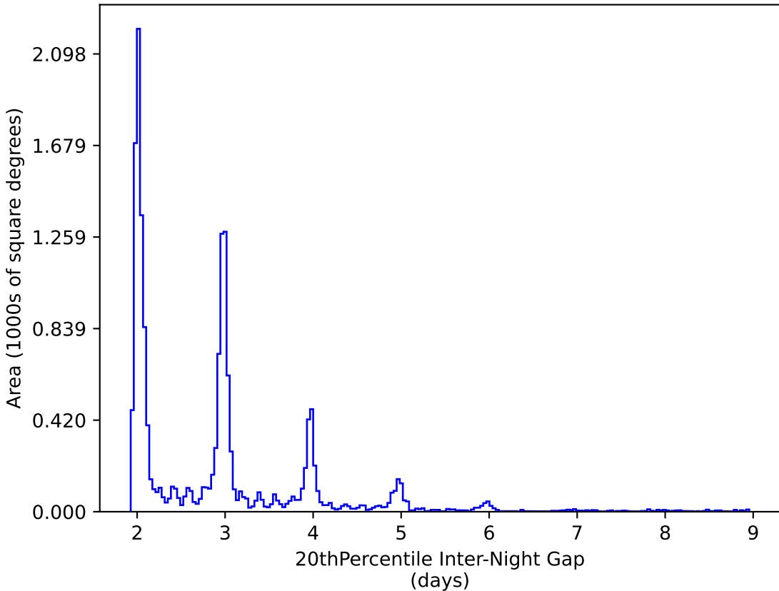
baseline_v2.1_10yrs WFD y band: 20thPercentile Inter-Night Gap
