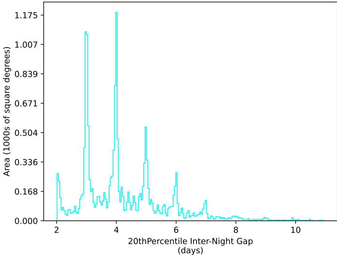
baseline_v2.1_10yrs WFD u band: 20thPercentile Inter-Night Gap
