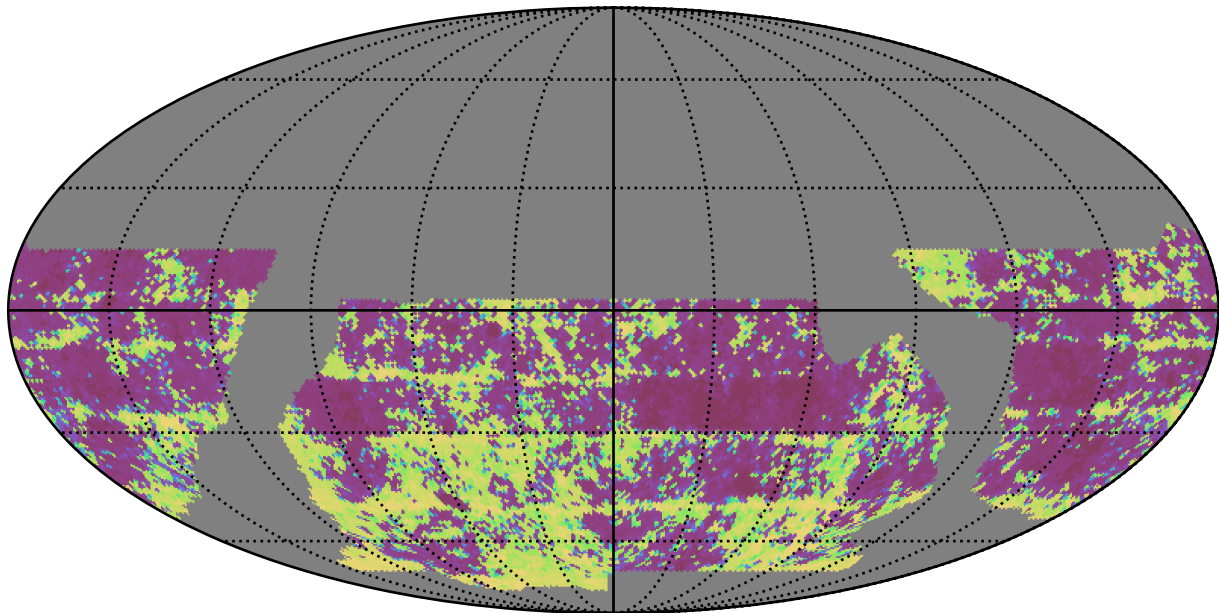
baseline_v2.1_10yrs WFD i band: 20thPercentile Inter-Night Gap
