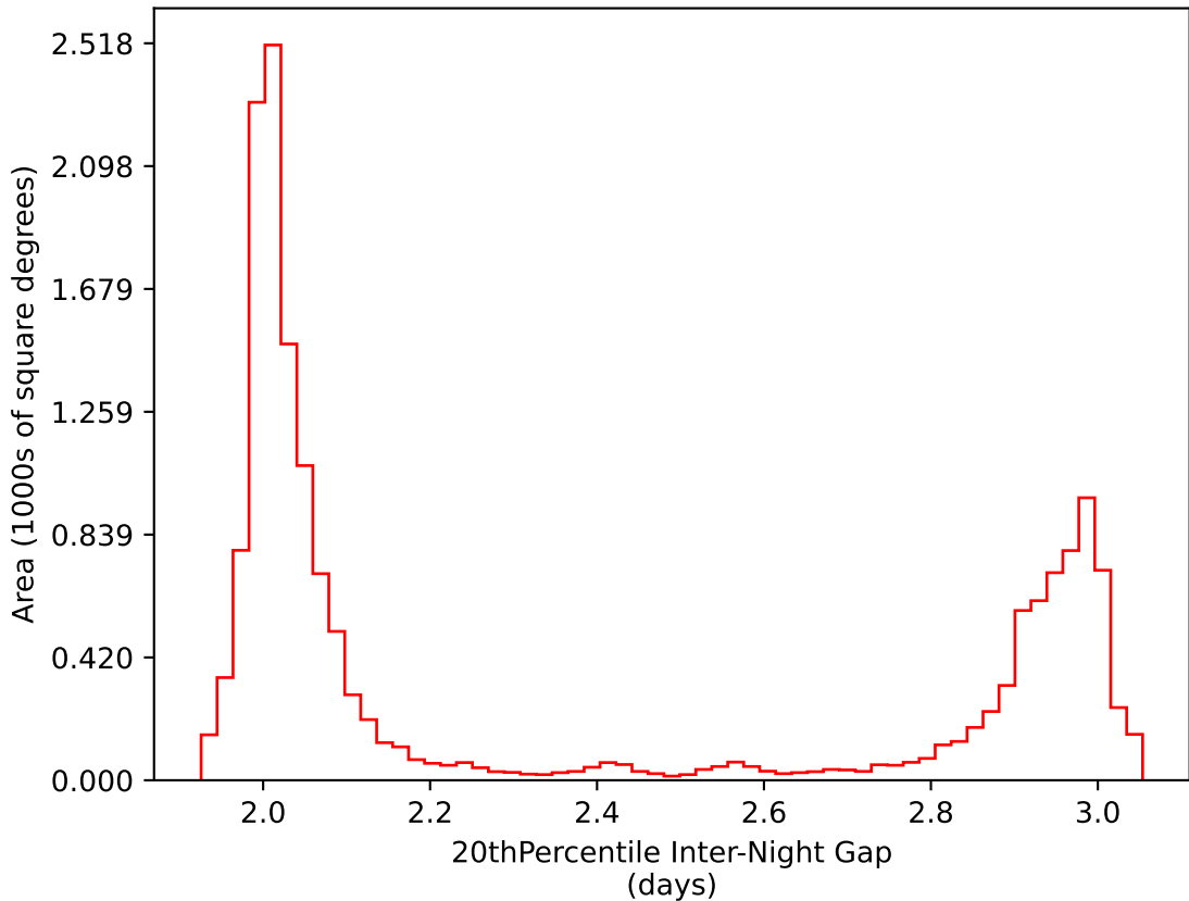
baseline_v2.1_10yrs WFD i band: 20thPercentile Inter-Night Gap
