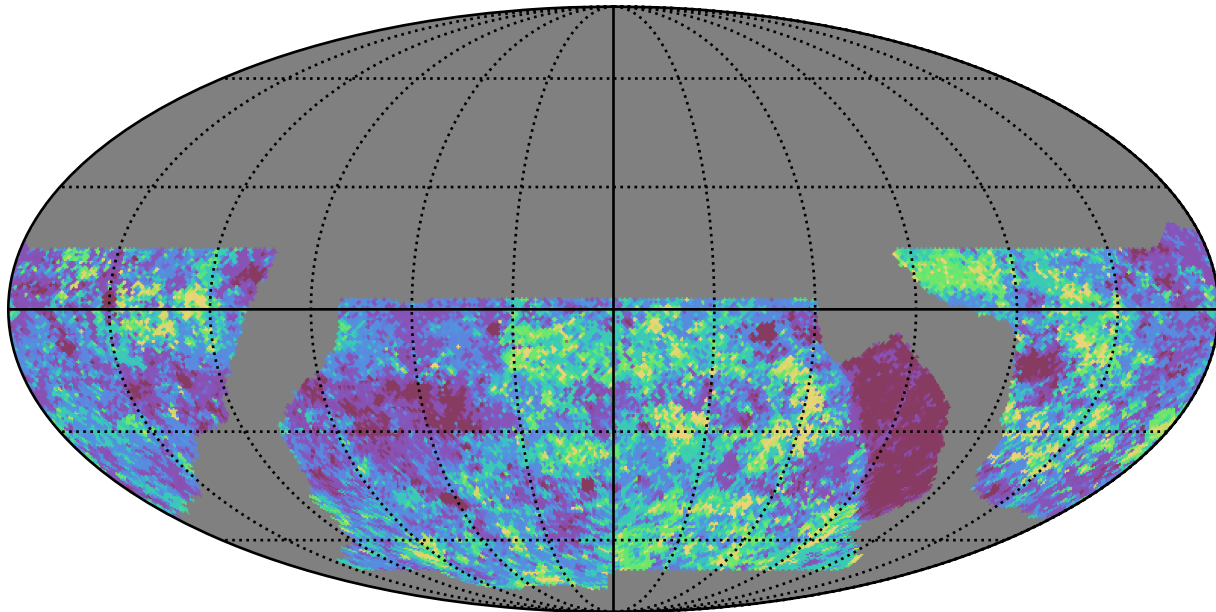
baseline_v2.1_10yrs WFD g band: 20thPercentile Inter-Night Gap
