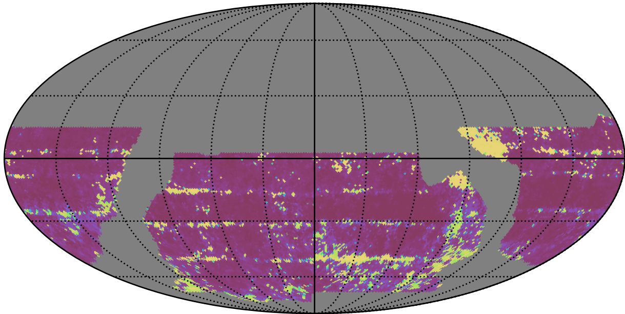
baseline_v2.1_10yrs WFD all bands: 20thPercentile Inter-Night Gap
