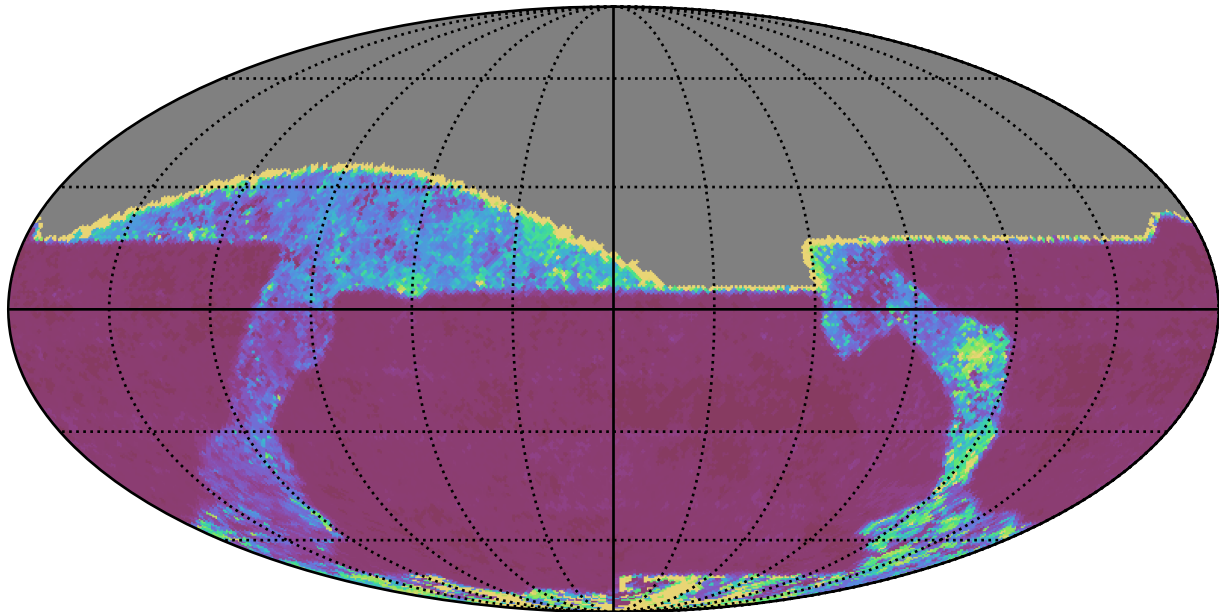
baseline_v2.1_10yrs All sky z band: 20thPercentile Inter-Night Gap
