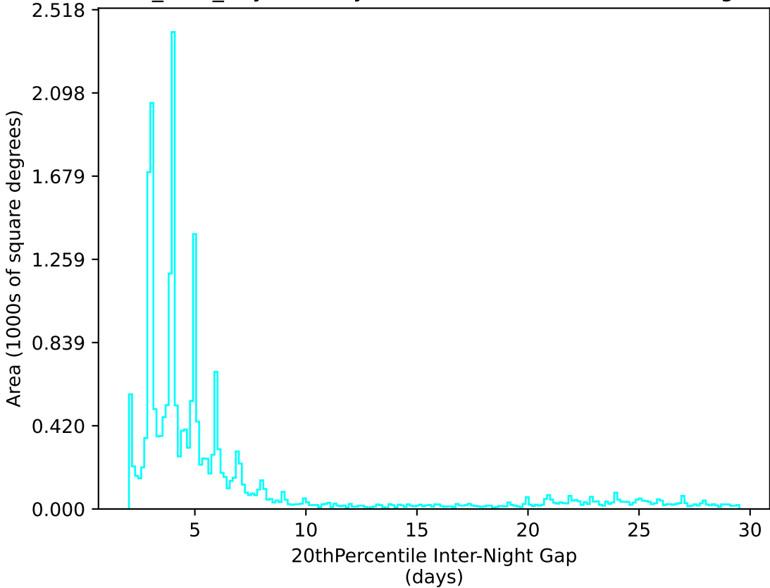
baseline_v2.1_10yrs All sky u band: 20thPercentile Inter-Night Gap
