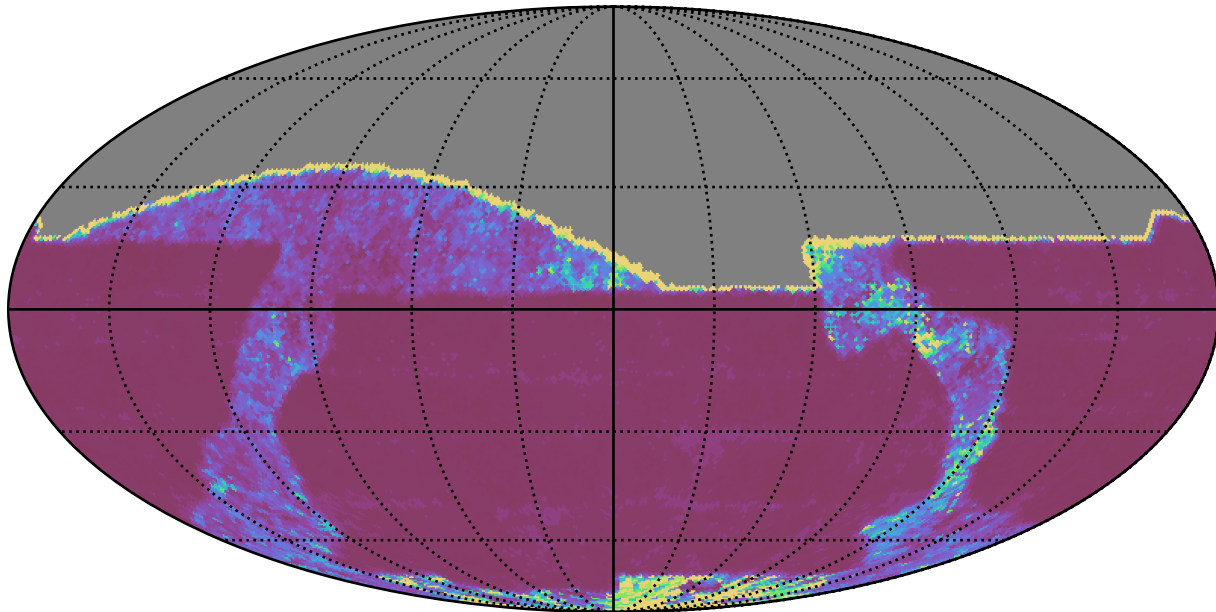
baseline_v2.1_10yrs All sky r band: 20thPercentile Inter-Night Gap
