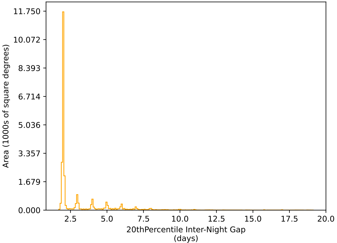
baseline_v2.1_10yrs All sky r band: 20thPercentile Inter-Night Gap
