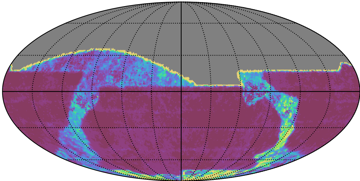
baseline_v2.1_10yrs All sky i band: 20thPercentile Inter-Night Gap
