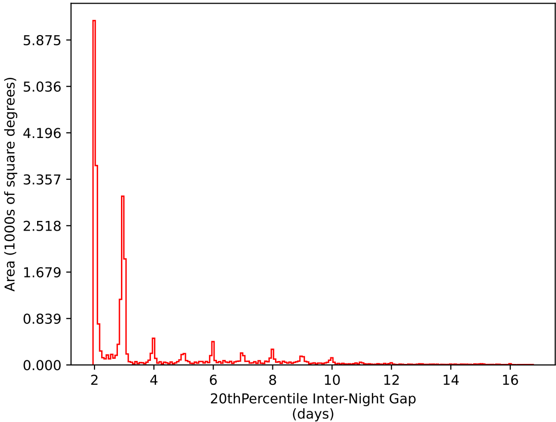
baseline_v2.1_10yrs All sky i band: 20thPercentile Inter-Night Gap
